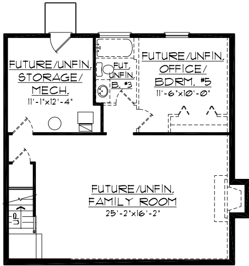
BASEMENT PLAN
