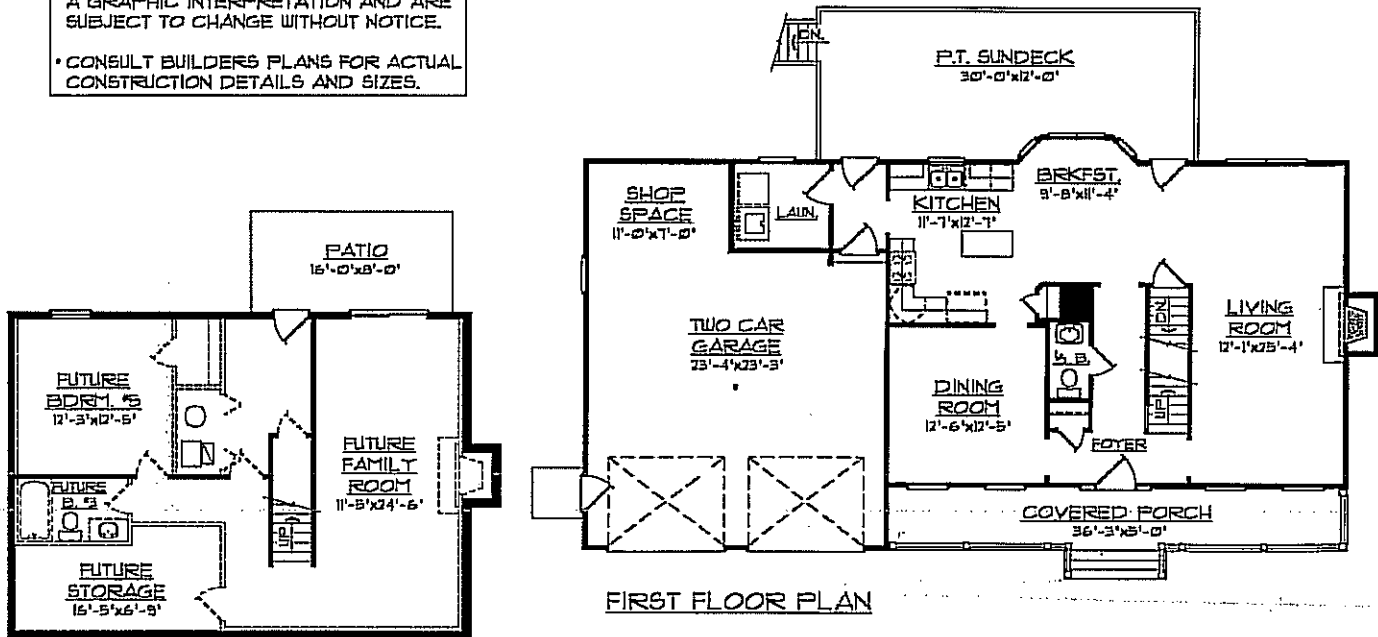
BASEMENT PLAN
