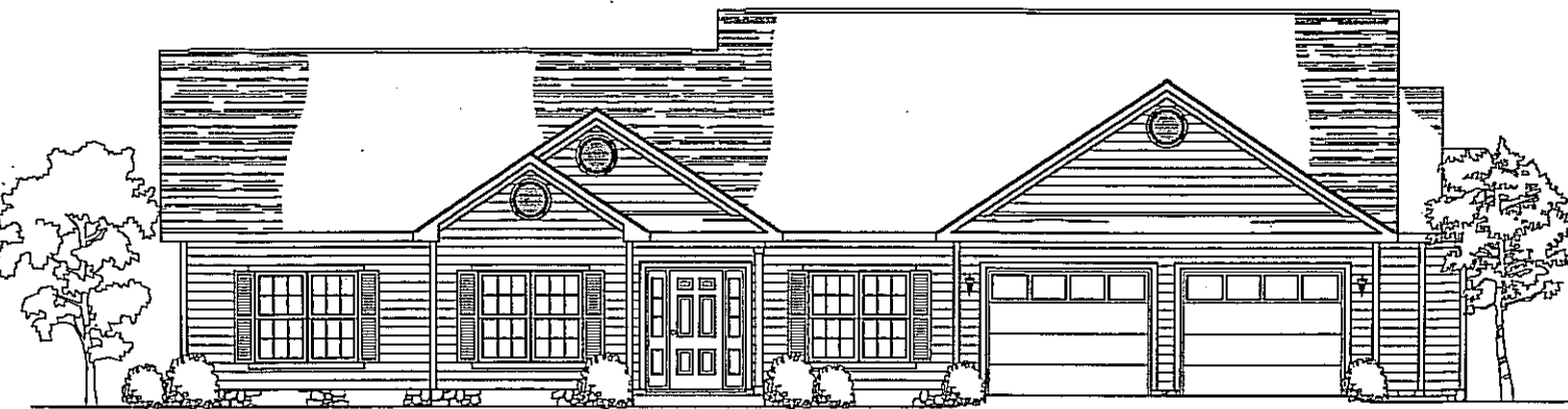
FRONT ELEVATION
