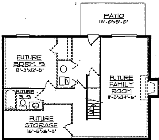
BASEMENT PLAN
