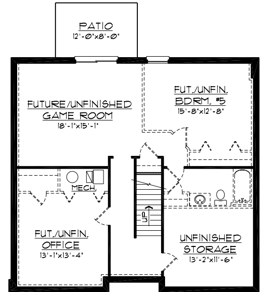
BASEMENT PLAN
