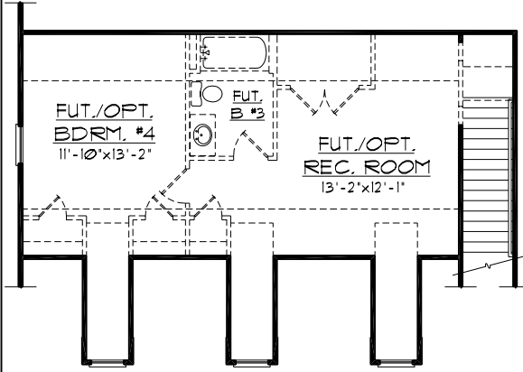
OPT. SECOND FLOOR PLAN
