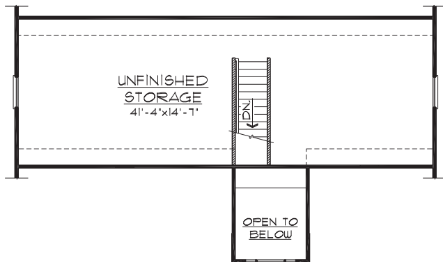
SECOND FLOOR PLAN OPTION "C"
