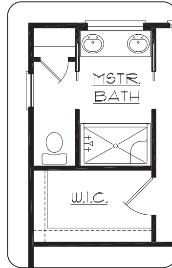
MASTER BATH PLAN OPTION "B" (FIBERGLASS WALK IN SHOWER)
