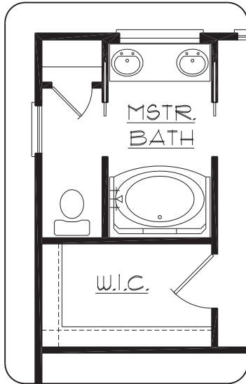
MASTER BATH PLAN OPTION "A" (FIBERGLASS SOAKING TUB/ SHOWER COMBINATION)
