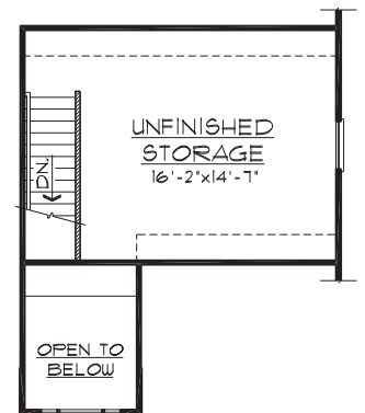
SECOND FLOOR PLAN OPTION "D"
