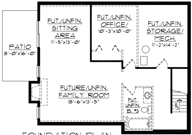
FOUNDATION PLAN
