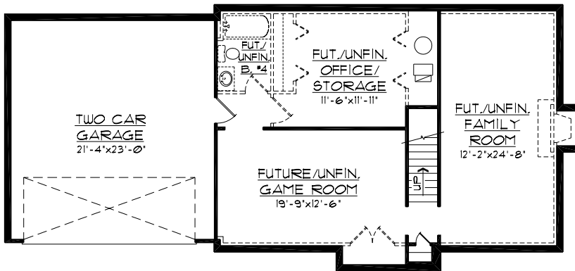
FOUNDATION PLAN
