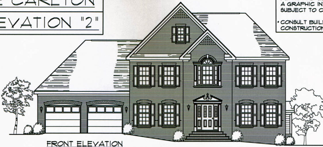
FRONT ELEVATION
