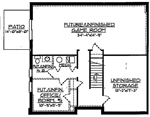
BASEMENT PLAN
